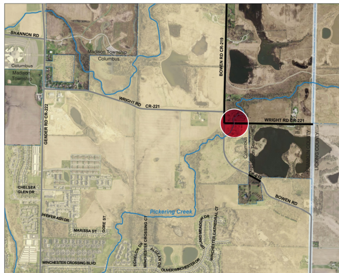
Wright Road Bridge 1.93 over Pickering Creek
