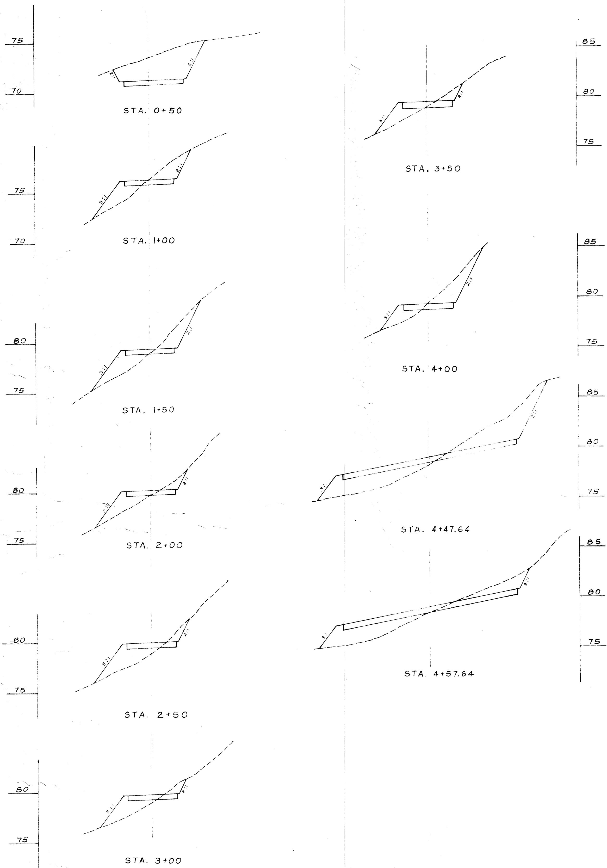
X-SECTIONS SCALES: HORIZ. 1" = 20' VERT. 1" = 5'
