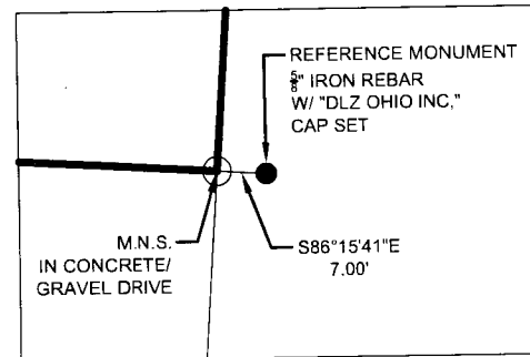
DETAIL A SCALE 1:30
