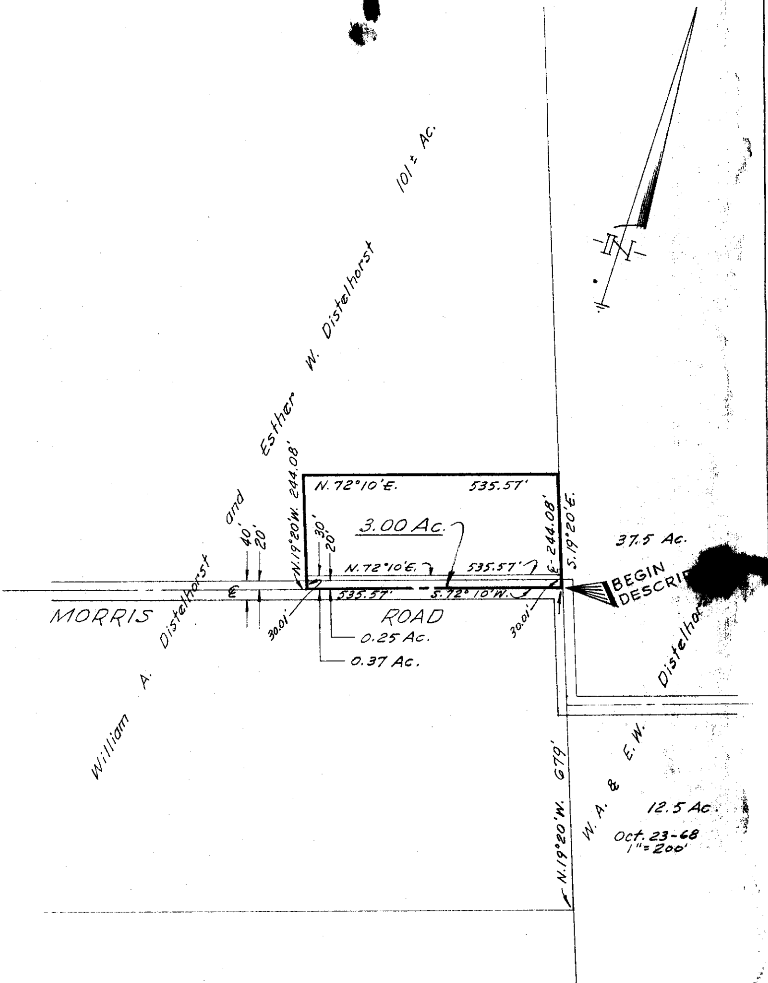
Plat showing a 3.00 Acre Tract, being part of the William A. Distelhorst and Esther W. Distelhorst 101± Acre Tract, part of Survey No. 2670, Virginia Military District, Brown Township, Franklin County, Ohio.
