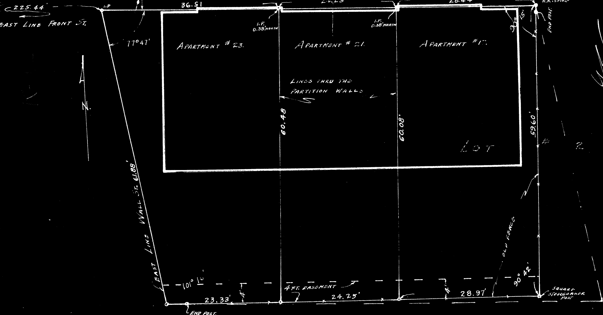
SURVEY OF WEST PART OF LOT 2, T. W. TALMADGE'S SOUTH ADDITION - P.B. 1, P. 412, RECORDER'S OFFICE, FRANKLIN CO., O. DATE DEC. 13, 1948. SCALE 1" = 10'. O = IRON STAKES.
